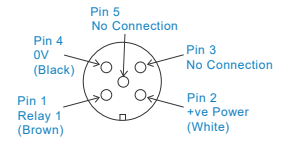
Connection Details Top & Bottom Connector
