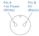
Connection Details
