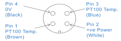
Connection Details
