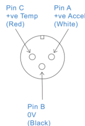
Connection Details
