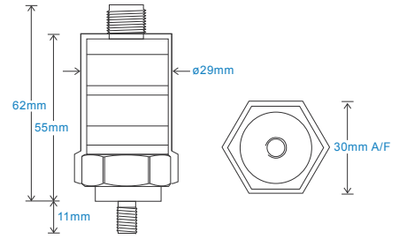
Dimensions with included protective cover
